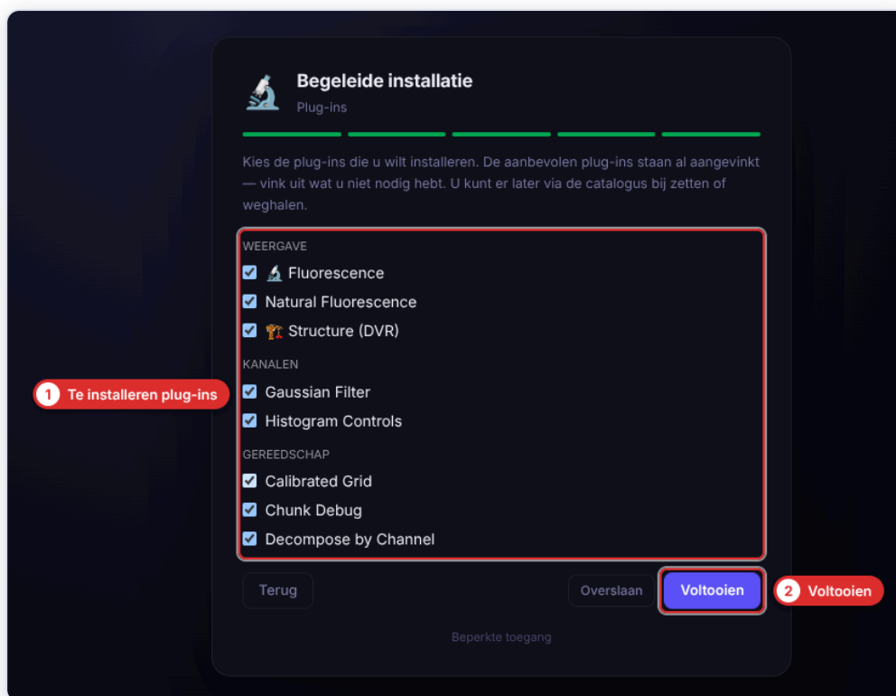
▲ Wizard, stap 5.
